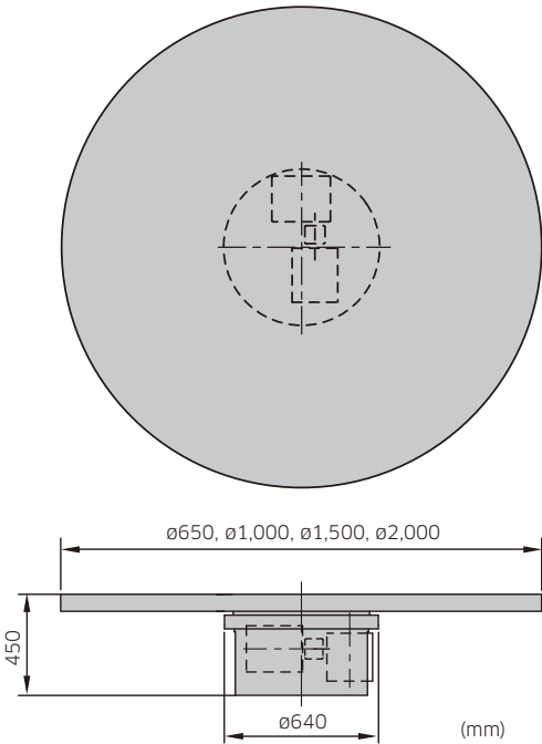
External View and Dimensions
