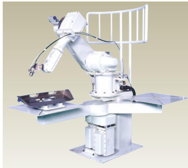
Servo twister + KF121
